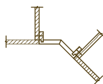
BASE & WALL CORNER FILLERS
