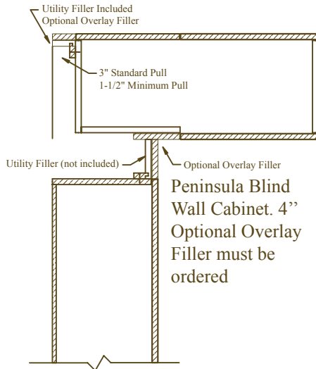
PENINSULA BLIND WALL CORNER DETAIL
