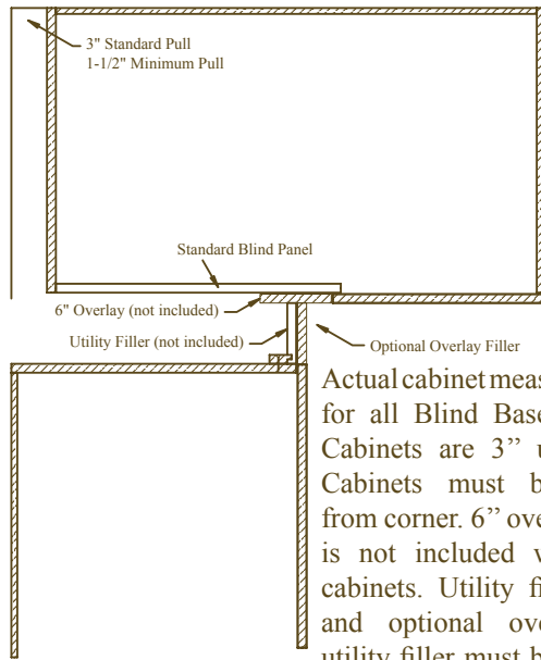
BLIND BASE OR WALL CORNER DETAIL
