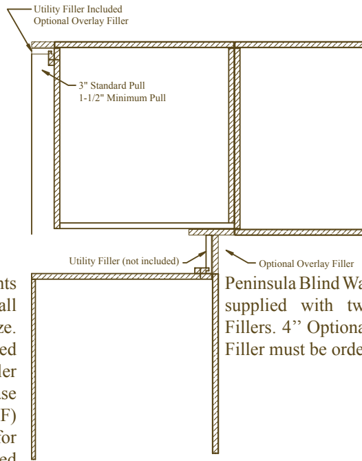
Universal Filler Application
